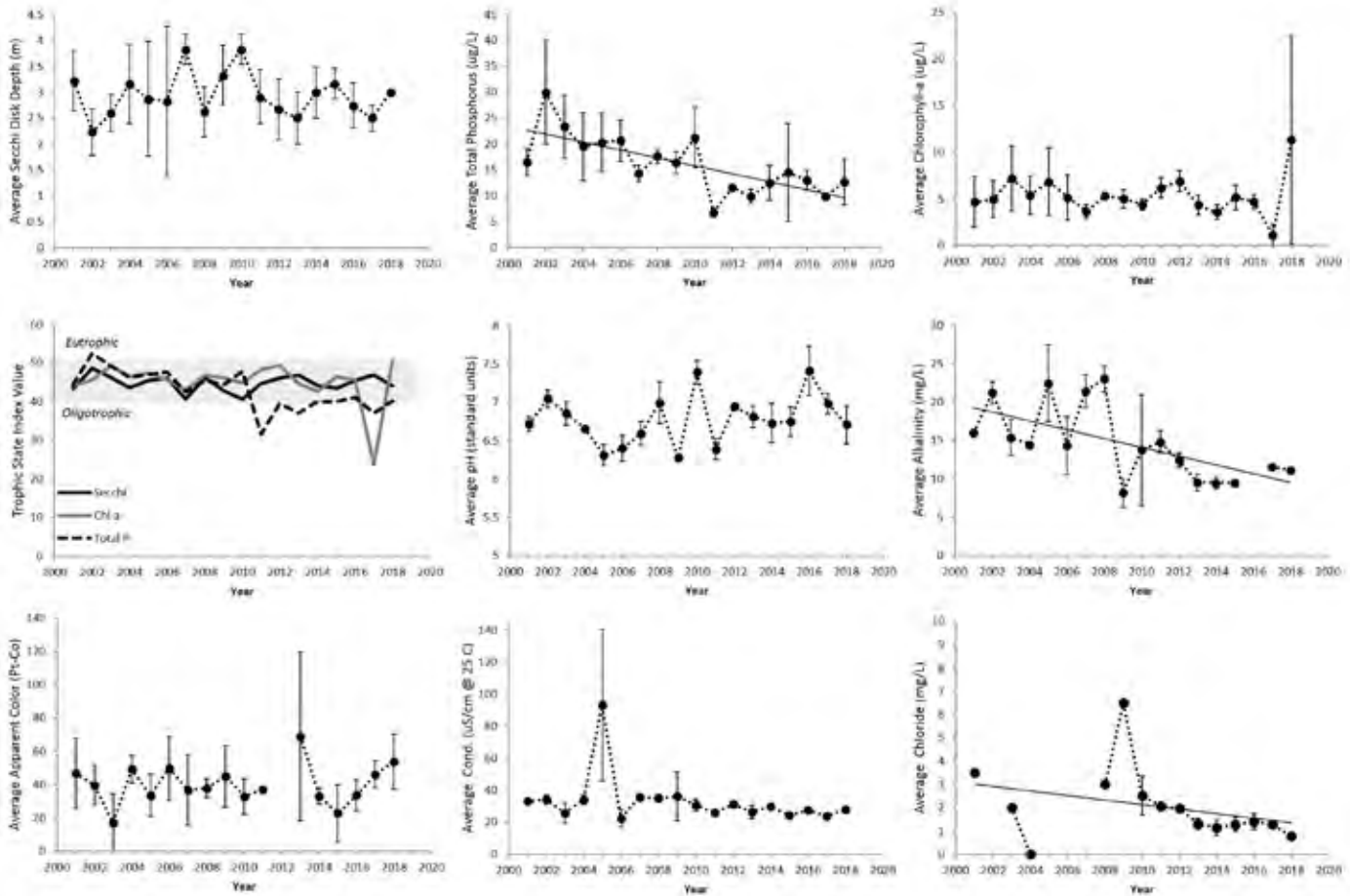
Annual average values of select water quality indicators for Lake of the Pines, 2001-2018. Vertical bars represent \pm 1 standard deviation of the mean; Solid trend lines across the data indicate a statistically significant trend ( p < 0.05 ).
