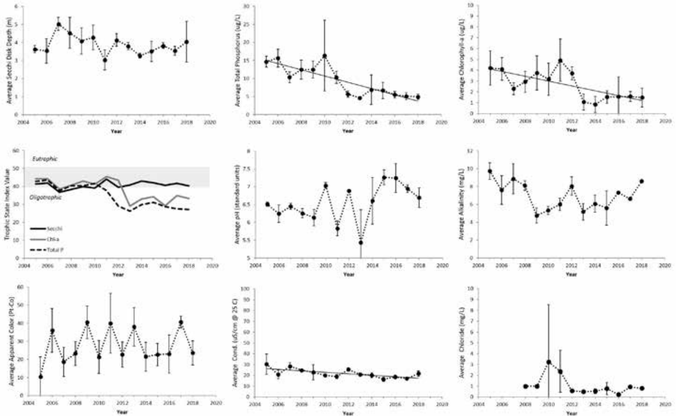
Annual average values of select water quality indicators for Moss Lake, 2005-2018. Vertical bars represent \pm 1 standard deviation of the mean; Solid trend lines across the data indicate a statistically significant trend ( p < 0.05 ).
