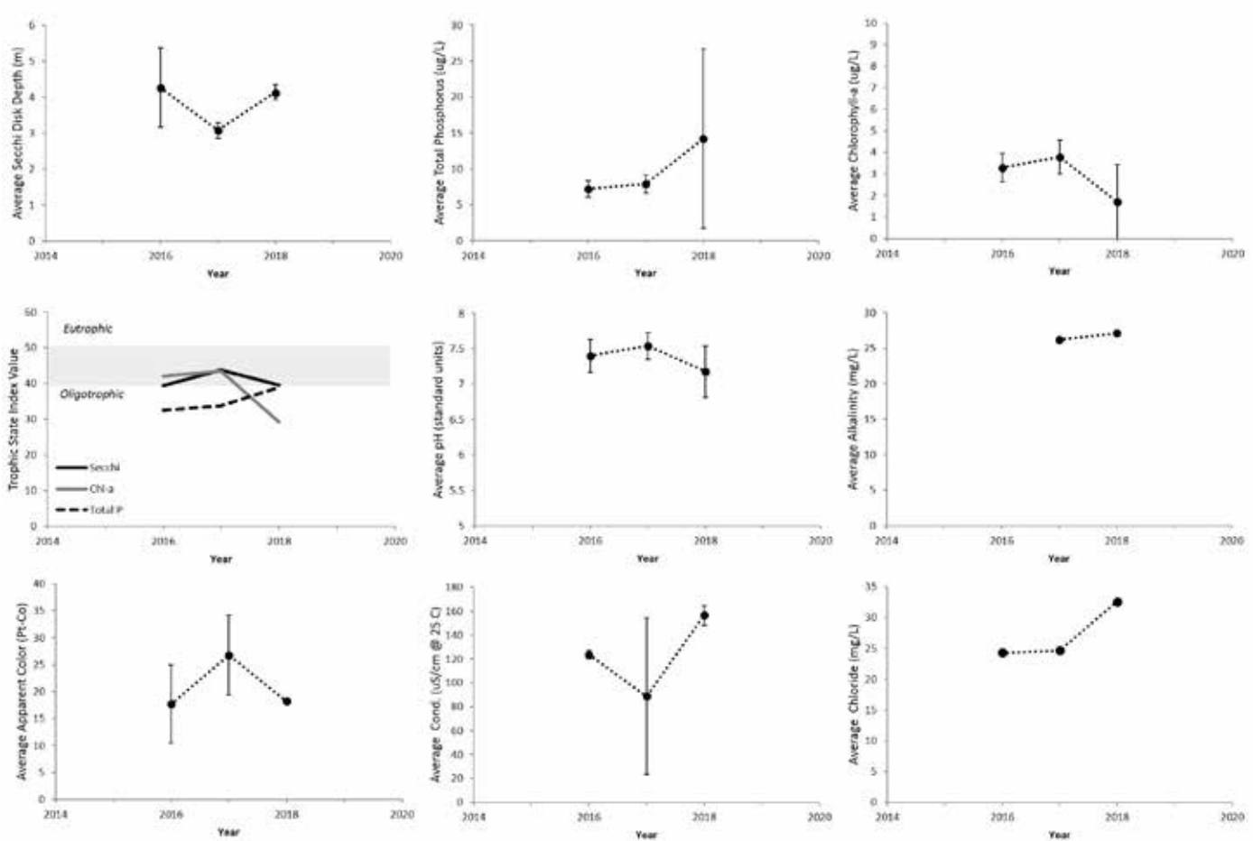
Annual average values of select water quality indicators for East Caroga Lake. Vertical bars represent \pm 1 standard deviation of the mean; Solid trend lines across the data indicate a statistically significant trend ( p < 0.05 ).
