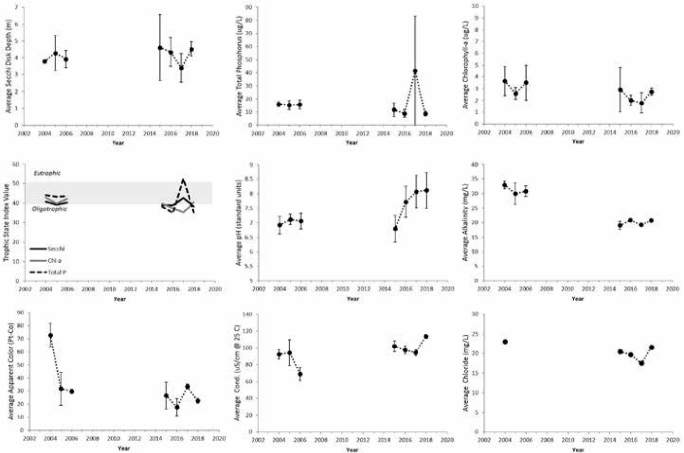
Annual average values of select water quality indicators for Loon Lake, 2004-2018. Vertical bars represent \pm 1 standard deviation of the mean; Solid trend lines across the data indicate a statistically significant trend ( p < 0.05 ).
