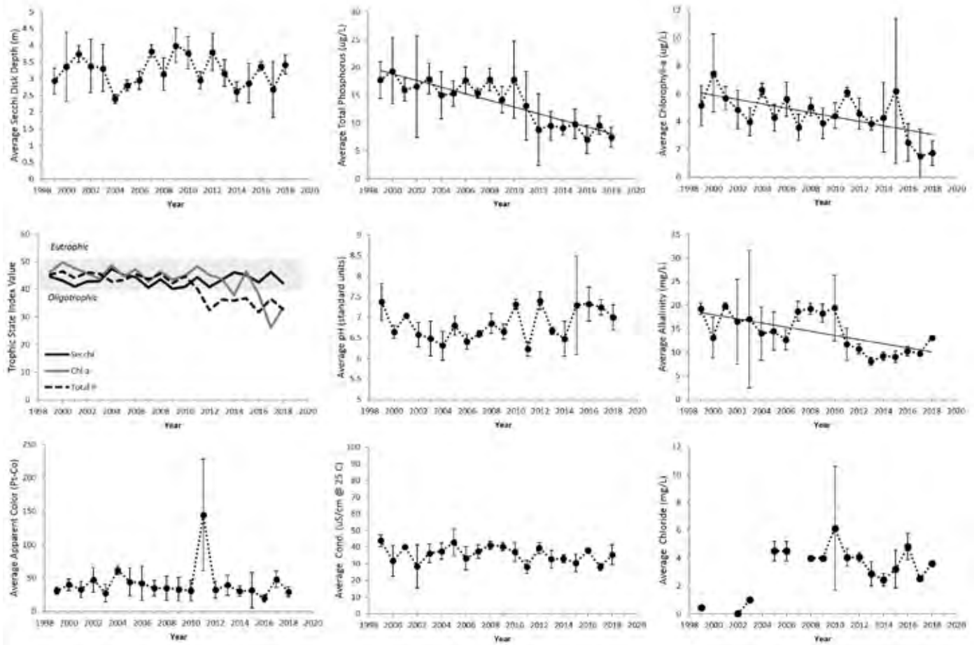
Annual average values of select water quality indicators for Stony Creek Pond, 1999-2018. Vertical bars represent \pm 1 standard deviation of the mean; Solid trend lines across the data indicate a statistically significant trend ( p < 0.05 ).
