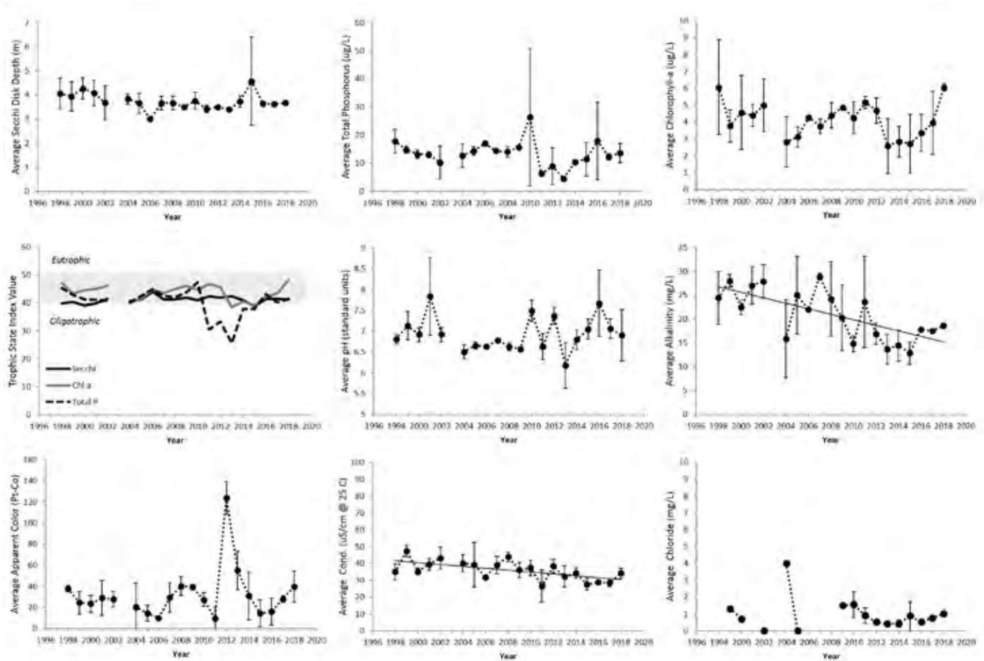
Annual average values of select water quality indicators for Eli Pond, 1998-2018. Vertical bars represent \pm 1 standard deviation of the mean; Solid trend lines across the data indicate a statistically significant trend ( p < 0.05 ).
