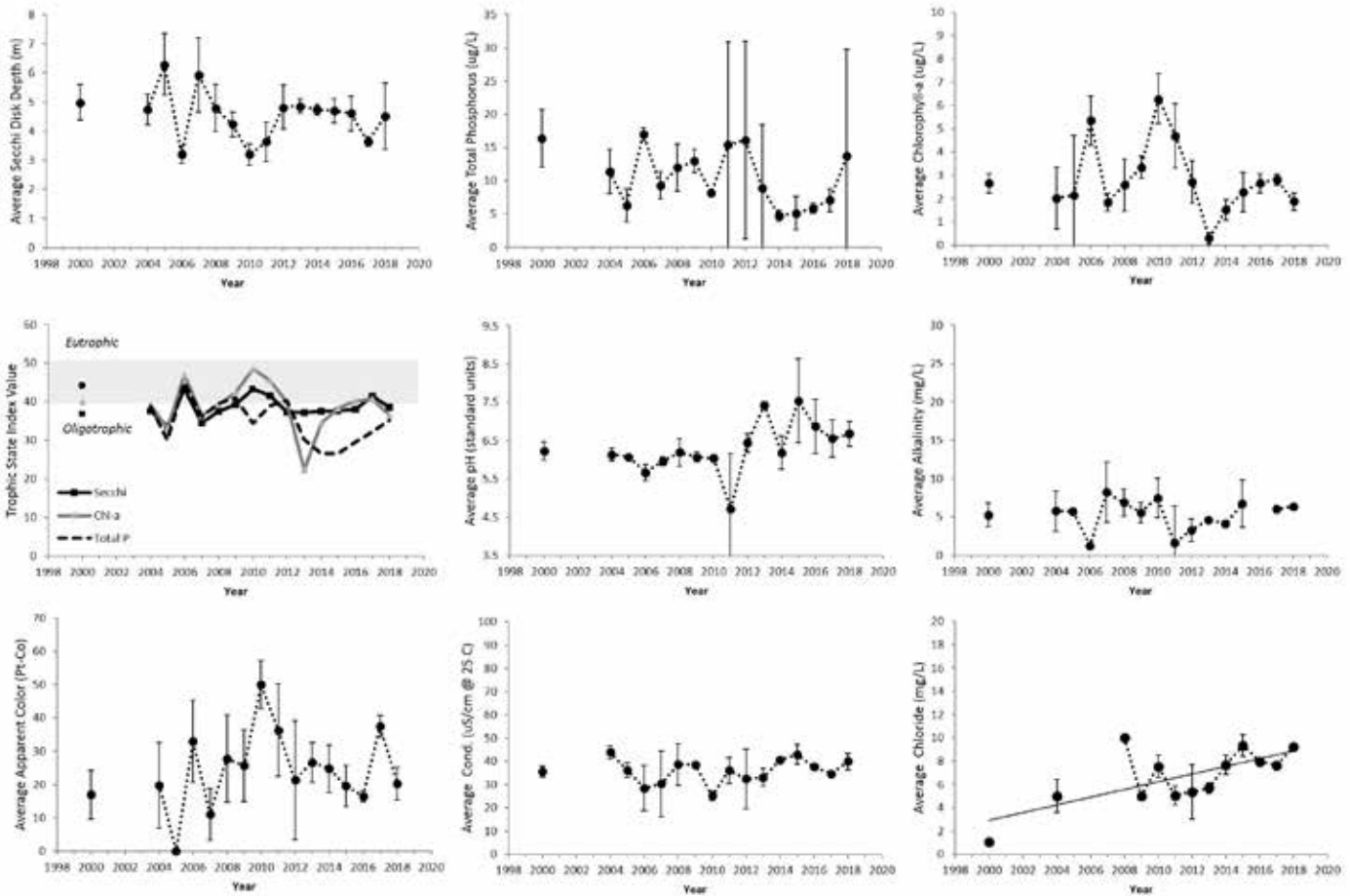
Annual average values of select water quality indicators for Canada Lake, 2000-2018. Vertical bars represent \pm 1 standard deviation of the mean; Solid trend lines across the data indicate a statistically significant trend ( p < 0.05 ).
