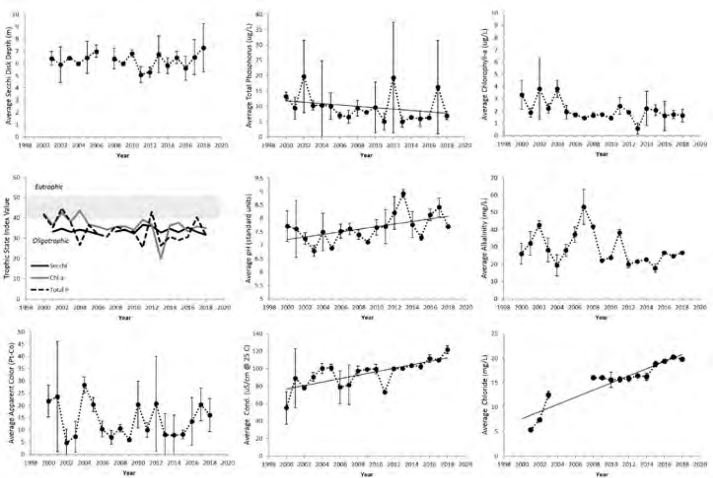
Annual average values of select water quality indicators for Trout Lake, 2000-2018. Vertical bars represent \pm 1 standard deviation of the mean; Solid trend lines across the data indicate a statistically significant trend ( p < 0.05 ).
