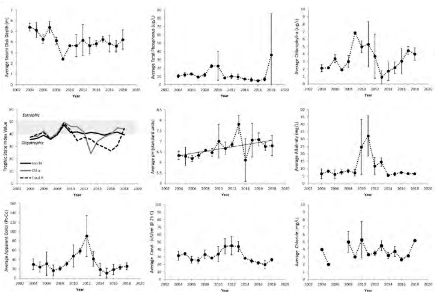
Annual average values of select water quality indicators for Indian Lake, 2004-2018. Vertical bars represent \pm 1 standard deviation of the mean; Solid trend lines across the data indicate a statistically significant trend ( p < 0.05 ).
