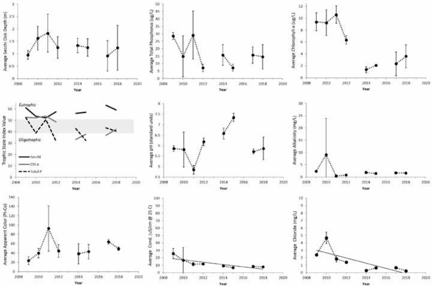
Annual average values of select water quality indicators for Otter Pond 2009-2018. Vertical bars represent \pm 1 standard deviation of the mean; Solid trend lines across the data indicate a statistically significant trend ( p < 0.05 ).
