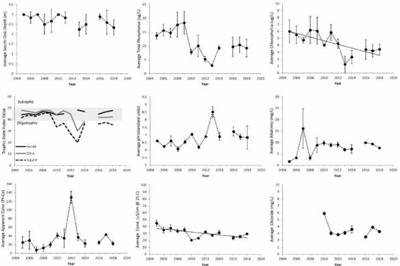
Annual average values of select water quality indicators for Lake Abanakee 2005-2018. Vertical bars represent \pm 1 standard deviation of the mean; Solid trend lines across the data indicate a statistically significant trend ( p < 0.05 ).
