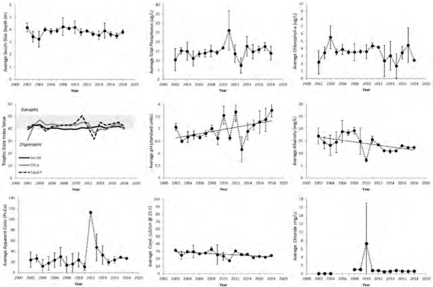
Annual average values of select water quality indicators for Garnet Lake, 2002-2018. Vertical bars represent \pm 1 standard deviation of the mean; Solid trend lines across the data indicate a statistically significant trend ( p < 0.05 ).
