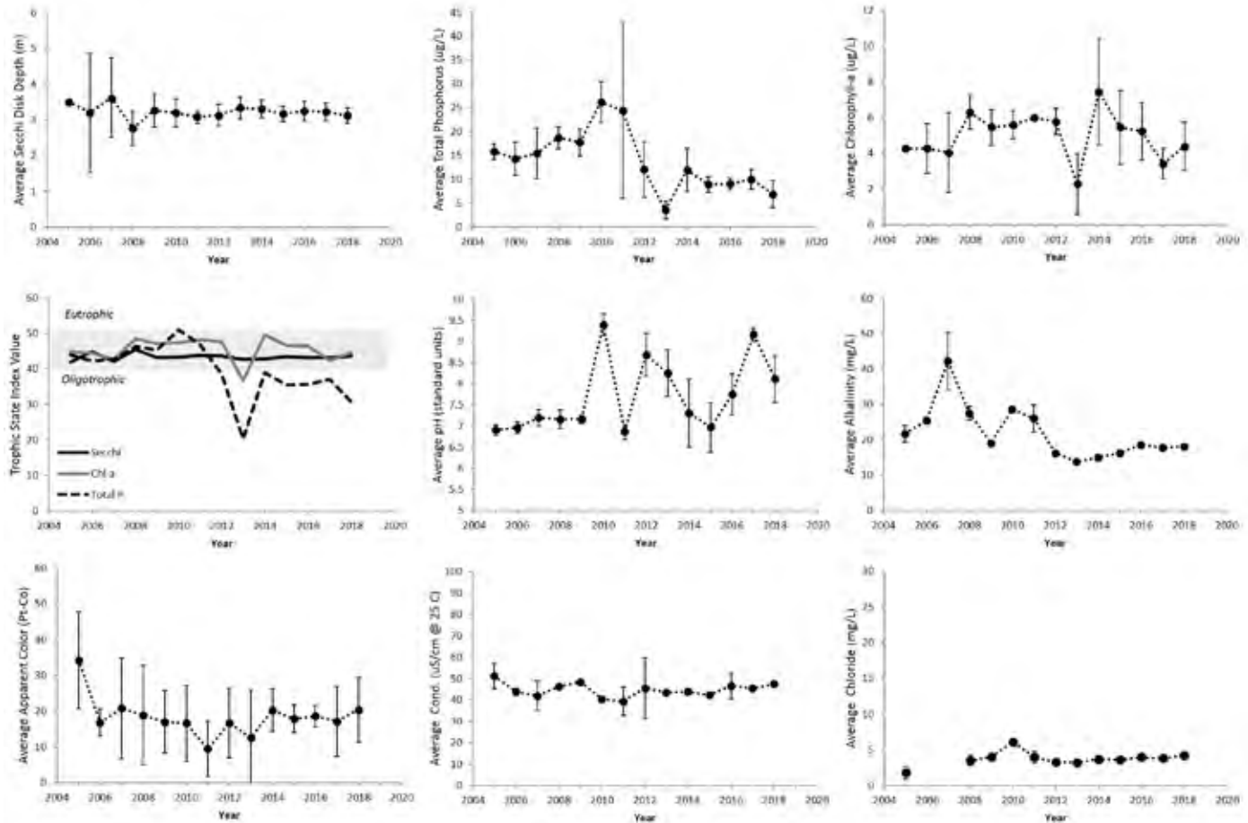
Lake wide annual average values of select water quality indicators for Fern Lake, 2005-2018. Vertical bars represent \pm 1 standard deviation of the mean; Solid trend lines across the data indicate a statistically significant trend ( p < 0.05 ).
