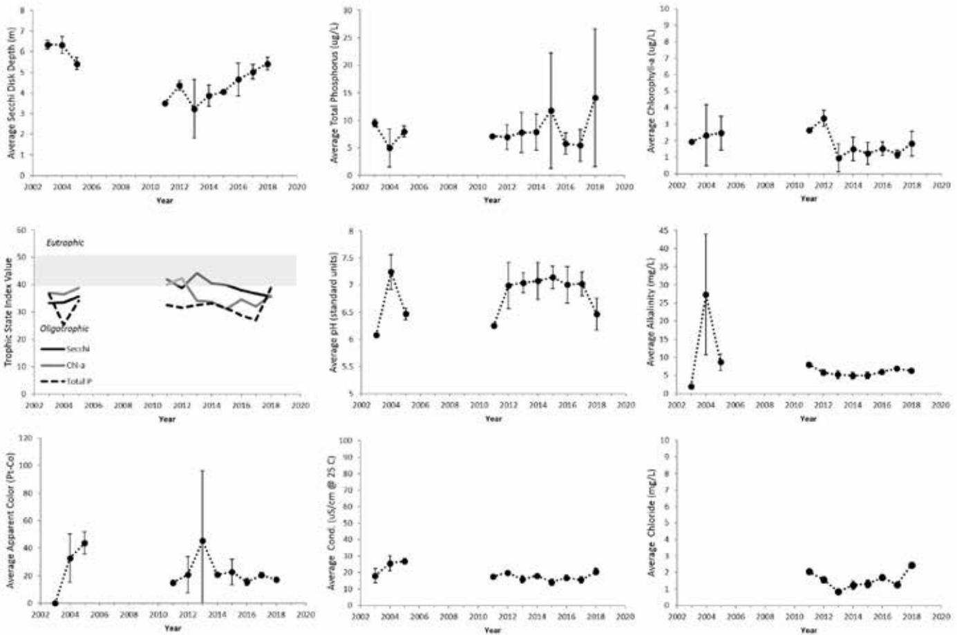
Annual average values of select water quality indicators for Chapel Pond, 2003-2018. Vertical bars represent \pm 1 standard deviation of the mean; Solid trend lines across the data indicate a statistically significant trend ( p < 0.05 ).
