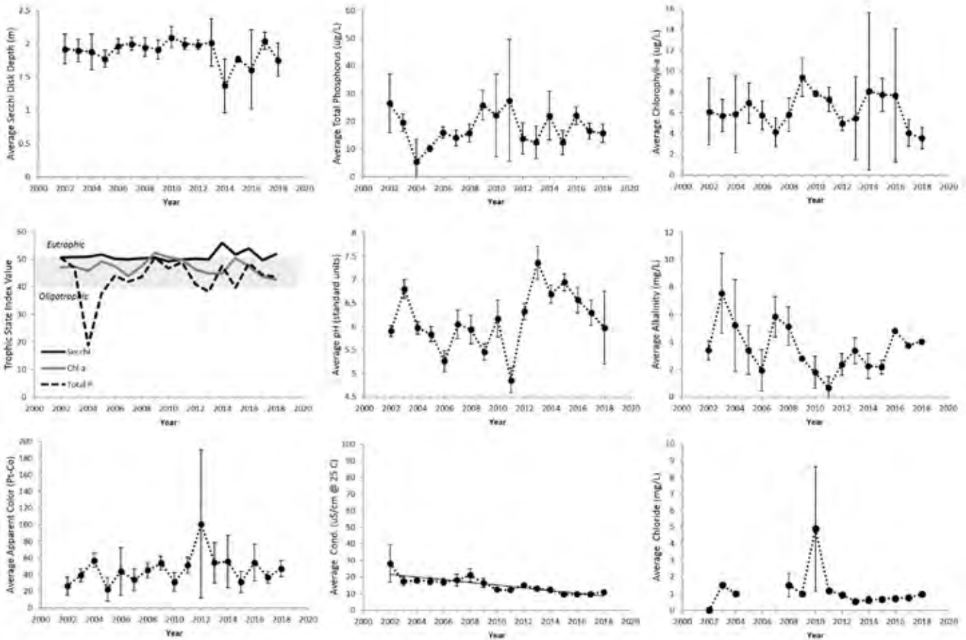
Annual average values of select water quality indicators for Lens Lake, 2002-2018. Vertical bars represent \pm 1 standard deviation of the mean; Solid trend lines across the data indicate a statistically significant trend ( p < 0.05 ).
