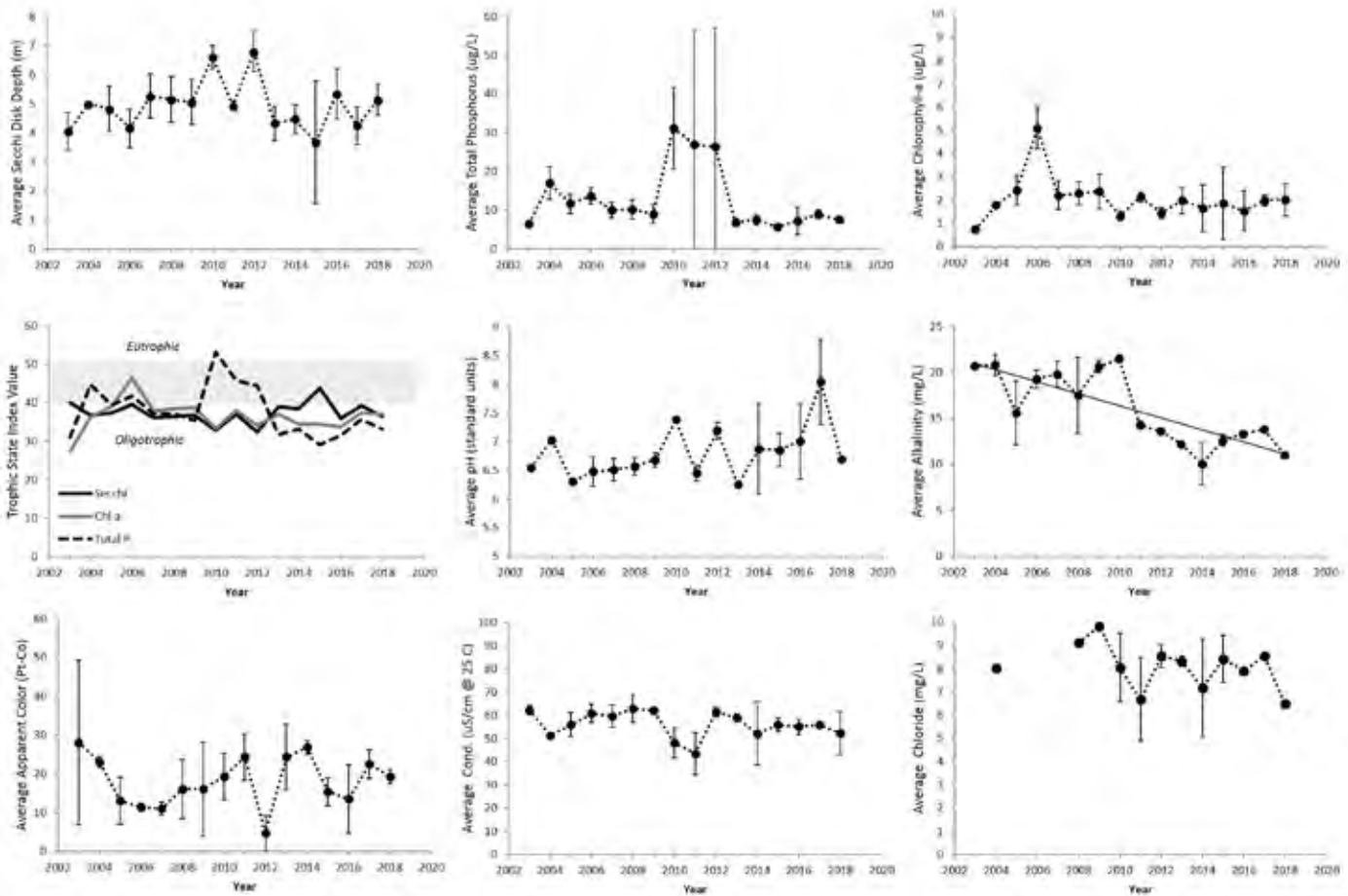
Annual average values of select water quality indicators for Kiwassa Lake, 2003-2018. Vertical bars represent \pm 1 standard deviation of the mean; Solid trend lines across the data indicate a statistically significant trend ( p < 0.05 ).
