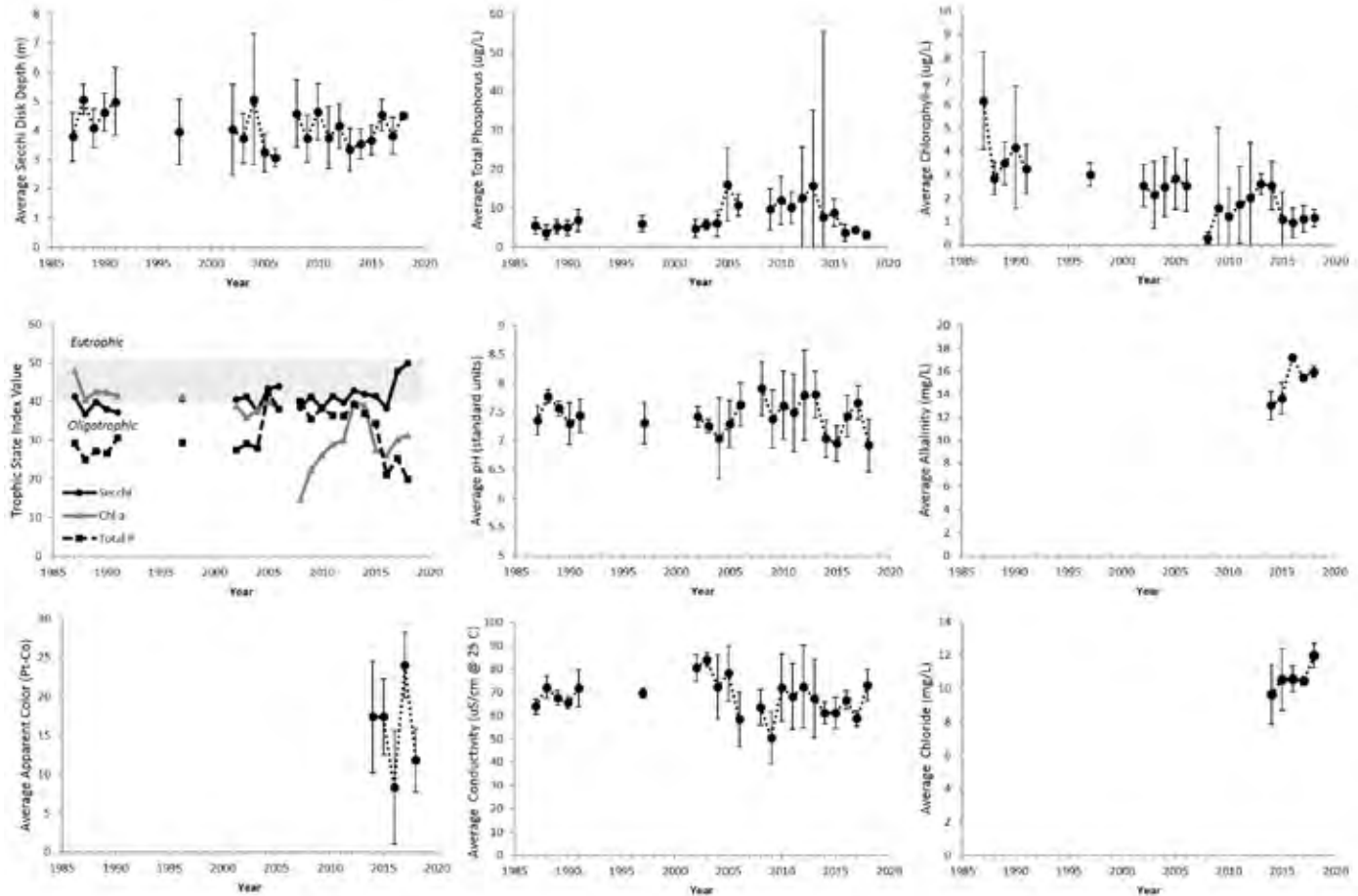
Lake wide annual average values of select water quality indicators for Schroon Lake, 1985-2018. Vertical bars represent \pm 1 standard deviation of the mean; Solid trend lines across the data indicate a statistically significant trend ( p < 0.05 ). Data from 1987-2013 form CSLAP, data from 2014-present from ALAP.
