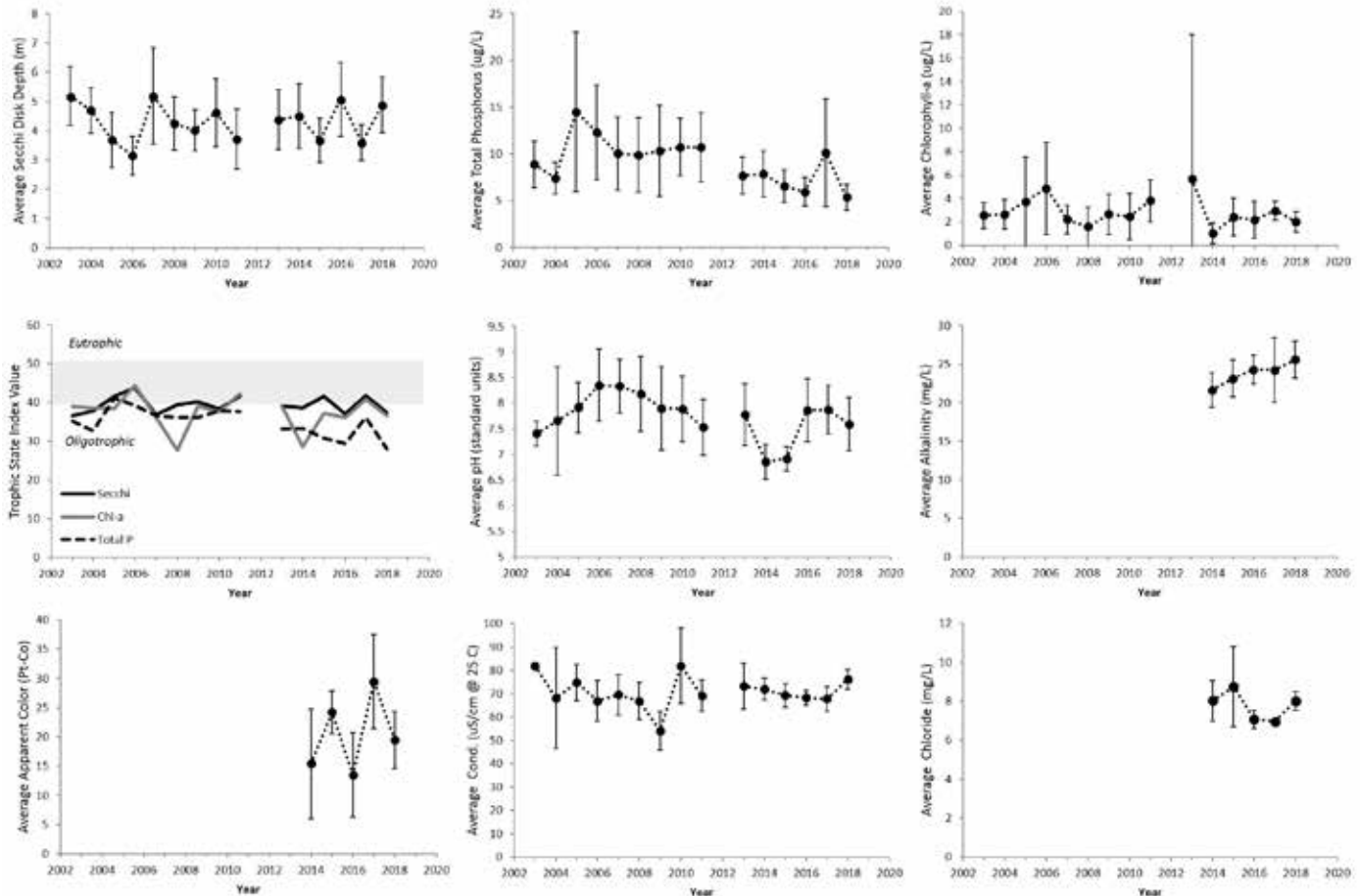
Lake wide annual average values of select water quality indicators for Paradox Lake, 2003-2018. Vertical bars represent \pm 1 standard deviation of the mean; Solid trend lines across the data indicate a statistically significant trend ( p < 0.05 ). Data from 2003-2013 from CSLAP, Data from 2014-present from ALAP.
