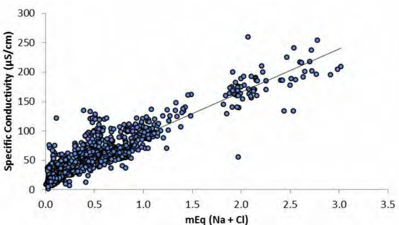
Figure 5. Relationship between conductivity and the combination of sodium and chloride in ALAP lakes, 2011-2017. ( P < 0.001 , R^2 = 0.86 , n = 1383 ).
